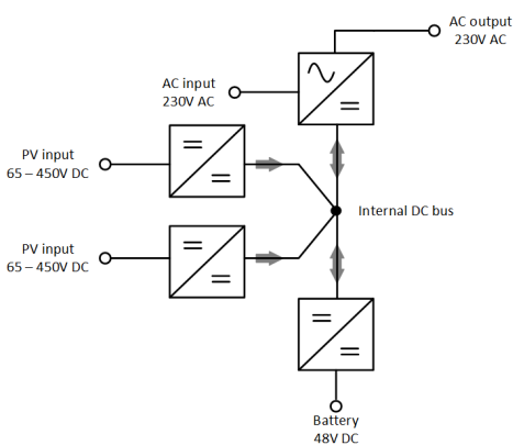
Multi RS19 Solarin rakenne
